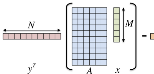
Figure 1: Inner product
